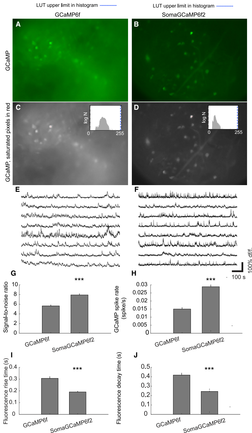
Figure 8. SomaGCaMP6f2 Improvements in Medial Prefrontal Cortex of Awake Mice Imaged with Endoscopic Microscopes
