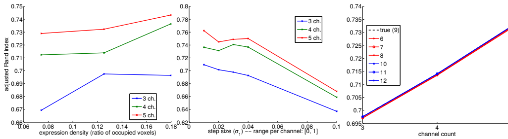
Supplementary Figure 7: Segmentation accuracy of simulated data a, Expression density (ratio of voxels occupied by at least one neuron) vs. ARI. b, \sigma_1 vs. ARI. c, Channel count vs. ARI for a 9-neuron simulation, where K \in [6, 12] . ARI is calculated for all voxels.
