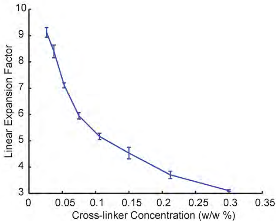
Figure S5. Expansion factor vs. cross-linking. Linear expansion factor for gels cast without specimens, as a function of the concentration of cross-linker used. Error bars represent standard deviation ( n = 4 samples).
