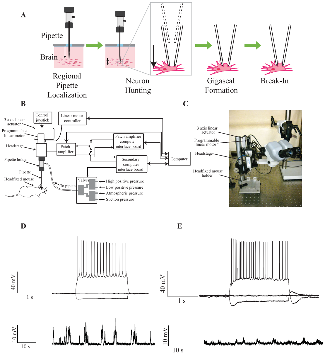
Figure 2. The autopatcher: a robot for in vivo patch clamping. (A) The four stages of the automated in vivo patch algorithm, discovered through iterative exploration of the parameters governing successful patch clamping: regional pipette localization, in which the pipette is lowered to a target zone in the brain; neuron hunting, in which the pipette is advanced until a neuron is detected via a change in pipette resistance; gigaseal formation, in which a gigaseal state is achieved (if cell-attached patching is desired, the algorithm can end here); break-in, in which the whole-cell state is achieved. (B) Schematic of a simple robotic system capable of performing the autopatching algorithm. The system consists of a conventional in vivo patch setup (i.e., pipette, headstage, three-axis linear actuator, patch amplifier plus computer interface board, and computer), equipped with a few additional modules: a programmable linear motor (to move the pipette up and down in a temporally precise fashion), a controllable bank of pneumatic valves for pressure control, and a secondary computer interface board to enable closed-loop control of the motor based upon sequences of pipette resistance measurements. (C) Photograph of the setup, focusing on three-axis linear actuator (with additional programmable linear motor) and the holder for head fixing the mouse. (D) Current clamp traces during current injection for a cortical neuron for which whole-cell state was established via the autopatcher. (E) Current clamp traces during current injection for a hippocampal neuron for which whole-cell state was established via the autopatcher. Adapted, with permission, from Kodandaramaiah et al. 53
